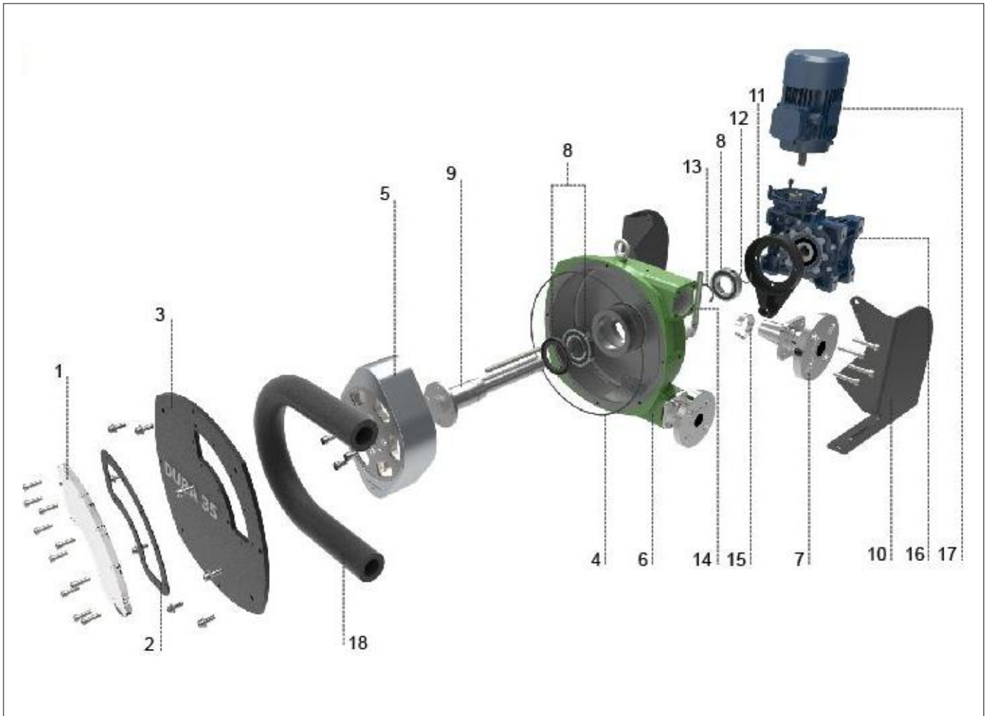
Figure 2 Layout (generic view)
