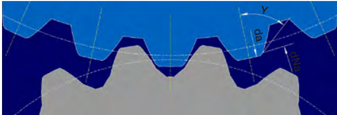
Topping cutter
