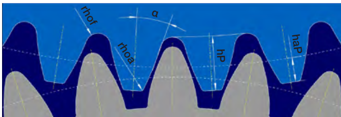
Basic rack tooth profile with topping
