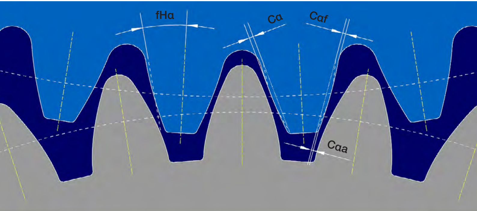
Pressure angle modification, Profile crowning, Addendum modification and Dedendum modification
