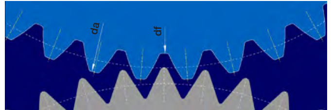
Block form and involute profiles for splines
